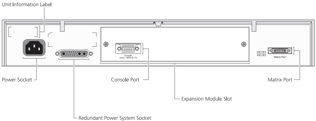
Figure 2 Switch 3300 FX — rear view
