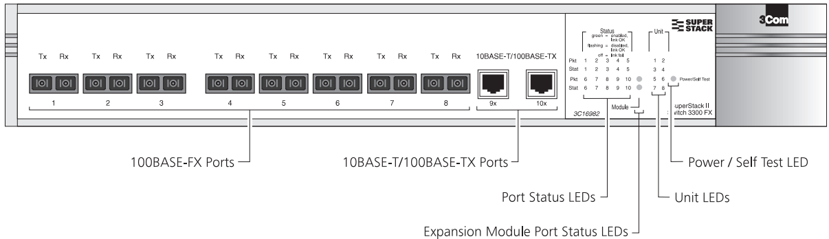
Figure 1 Switch 3300 FX — front view
