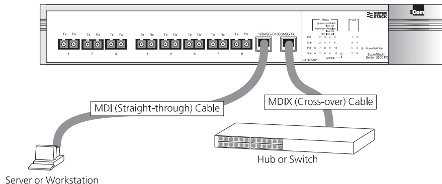
Figure 10 Connecting other devices to the Switch 3300 FX
