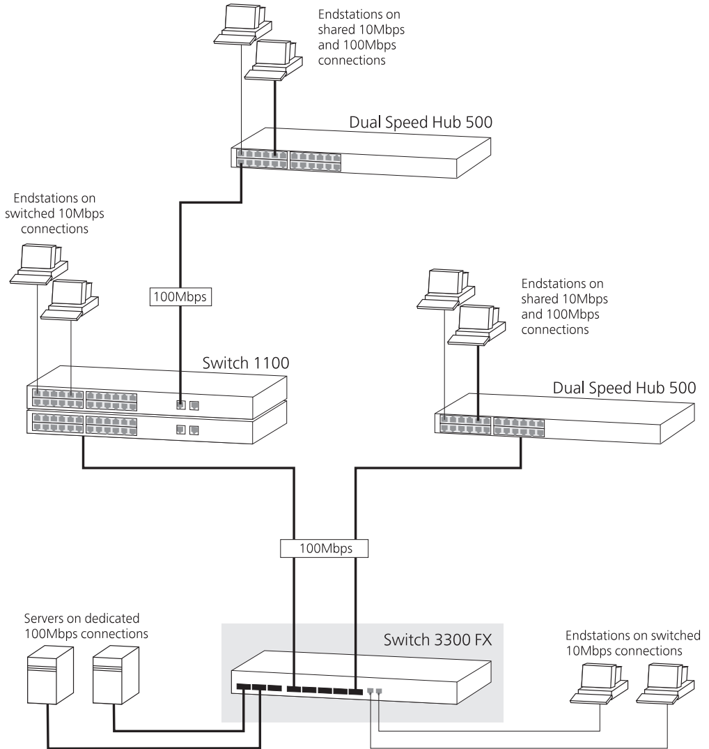
Figure 4 Using the Switch as a collapsed backbone
