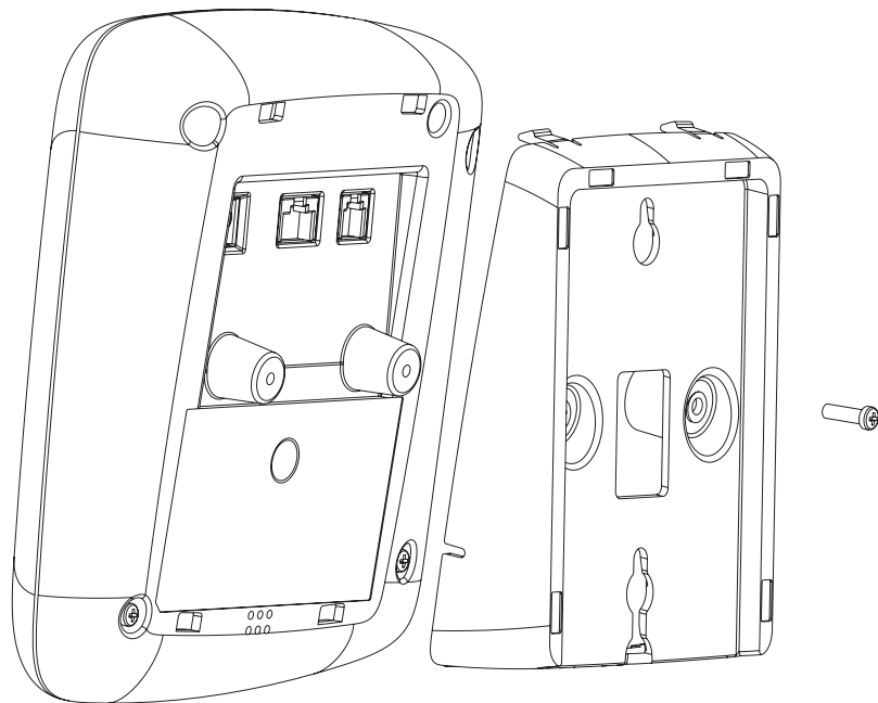
Figure 8 Wall-Mount Position
