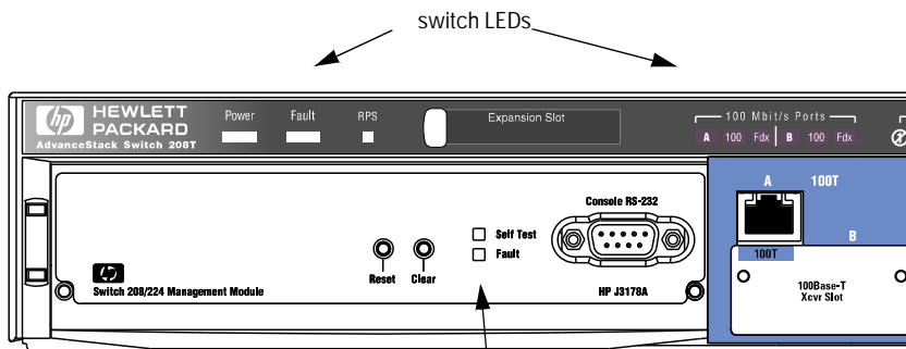
Switch Management Module LEDs
